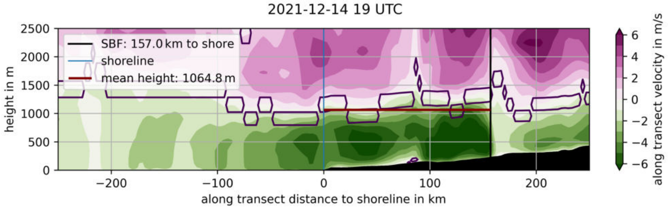
Figure 5.23: Along-transect wind velocity in the averaged cross-sections between 3.5^{\circ} and 3.9^{\circ} E on 14 December 2021 at 19 UTC. The purple contours show areas where the wind reversal criteria of Wexler (1946) is fulfilled, thus areas with zero horizontal wind. The brown line shows the mean SB height calculated between the shoreline (blue vertical line) and the SBF (black vertical line) (orography is subtracted).
