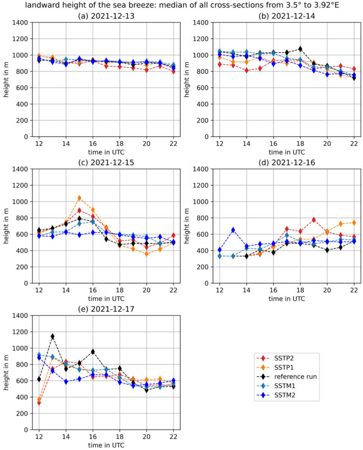
Figure 5.40: Landward Sea Breeze height, one plot for every day of the simulation period. The depicted height is the median of the heights calculated in each cross-section between 3.5° and 3.92°E in the case study area in West Nigeria.
