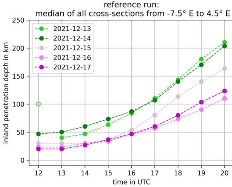
Figure 5.22: Hourly median of the inland penetration distance of the SB along all cross-sections from -7.5^\circ to 4.5^\circ E. The colours indicate the day of the reference run.
