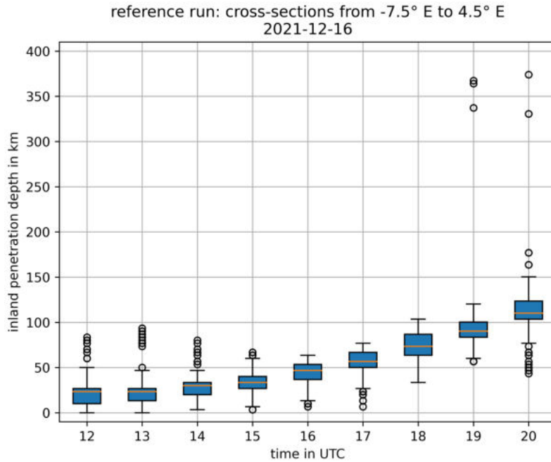
Figure 8.11: Hourly median of the inland penetration distance of the SB along all cross-sections from -7.5^\circ to 4.5^\circ E on 16 December 2021. The box extends from the first quartile to the third quartile. The whiskers extend from the box to the farthest data point lying within the 1.5 of the inter-quartile range.
