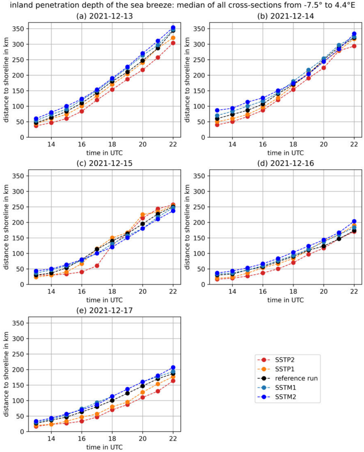
Figure 5.38: Median inland penetration distance of the SBF between -7.5^\circ and 4.4^\circ\text{E} (Ivory Coast to West Nigeria) for each day of the case study and for the reference run and the different SST experiments.
