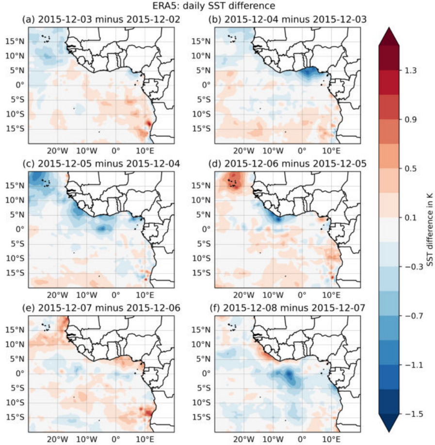
Figure 5.5: ERA5 data: SST difference from day to day during the SST drop from 02.12.2015 to 08.12.2015.
