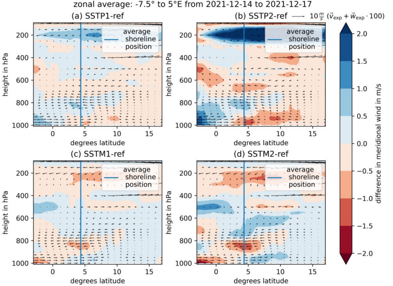
Figure 5.29: Comparison of the meridional wind velocity of the SST experiments to the reference run. The graphic compares the mean meridional wind component from a zonal mean between -7.5° and 5°E averaged from 14 to 17 December 2021. Blue shading indicates increased onshore winds and red shading increased offshore wind velocity in the SST experiment.
