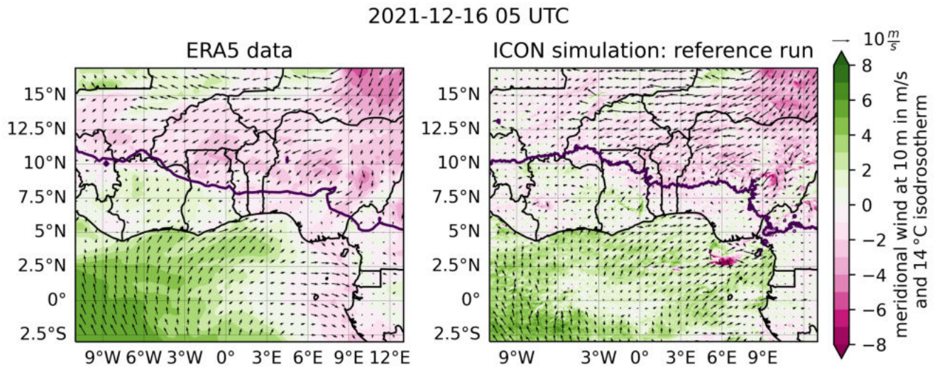
Figure 8.4: Comparison of the ERA5 dataset and the ICON reference run on 16 December 2021 at 5 UTC. Both graphics show arrows of the 10m wind speed and direction and the 10m meridional wind in the contours.
