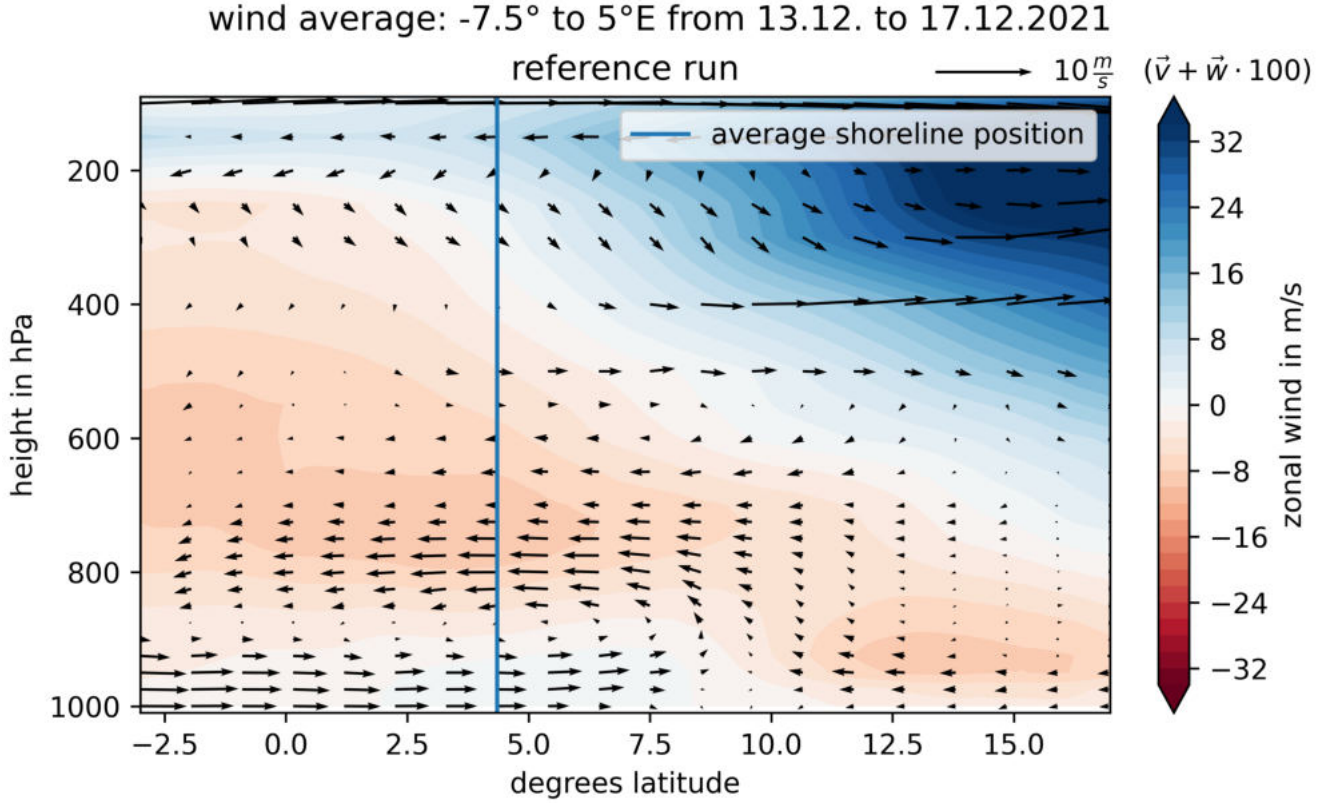
Figure 5.9: Meridional vertical wind profile averaged from 13 to 17 December 2021 in the reference run. The zonal mean was performed between -7.5^\circ and 5^\circ E. The arrows indicate the meridional and vertical wind components, whereby the vertical velocity is multiplied by a factor of 100. The contours depict the mean zonal winds in this area. In this zonal average, the land lies on average north of the blue vertical line (averaged latitudinal shoreline position).
