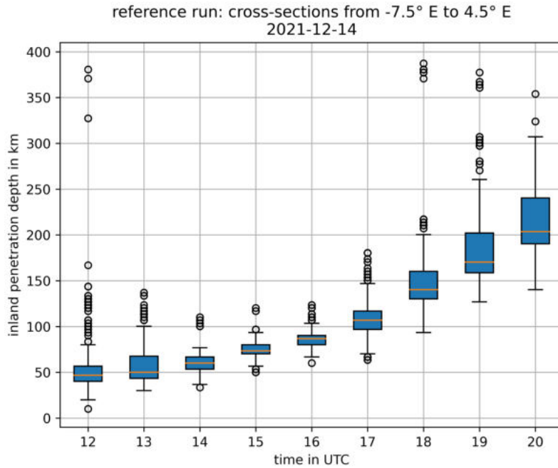
Figure 8.9: Hourly median of the inland penetration distance of the SB along all cross-sections from -7.5^\circ to 4.5^\circ E on 14 December 2021. The box extends from the first quartile to the third quartile. The whiskers extend from the box to the farthest data point lying within the 1.5 of the inter-quartile range.
