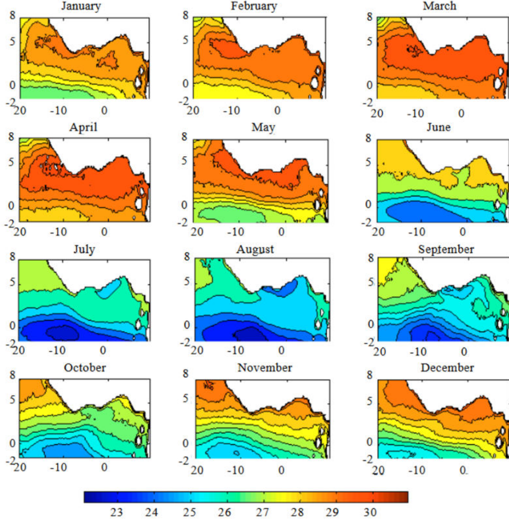
Figure 2.8: Spatial evolution of the monthly SSTs in the Guinea Gulf from 1998-2007 from Ali et al. (2011).
